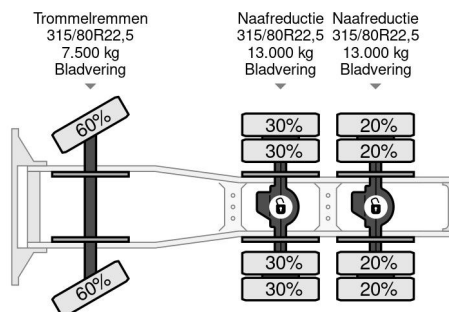
MAN 33.373 DFT 6x4 FULL STEEL SUSPENSION (13.000 A... Referenznummer: SN 59167518 Z
