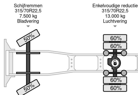
MAN TGX 18.440 BLS XLX (ZF16 MANUAL GEARBOX ... 4x2
