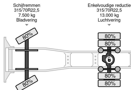
Volvo FH 460 GLOBETROTTER-XL (12+2 GEARS MA... 4x2
