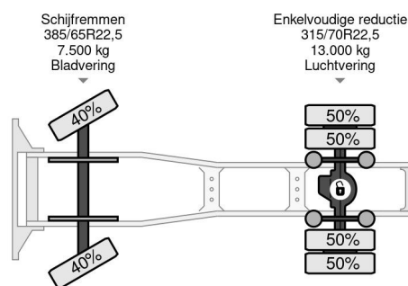
DAF XF 105.460 SPACECAB 4x2 (EURO 5 / AS-TRONIC / ZF...
