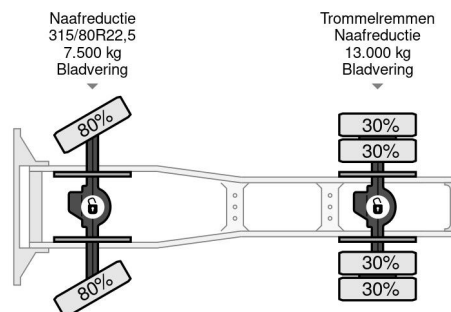
Mercedes-Benz Actros 2040 AS 4x4 FULL STEEL SUSPENS... Referentienummer: SN 57922171 Z
