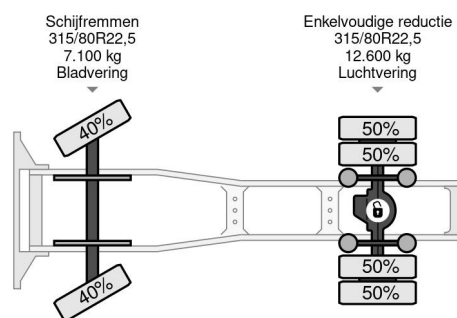
Renault Magnum 440 E-TECH (MACK ENGINE / ZF16 ... 4x2
