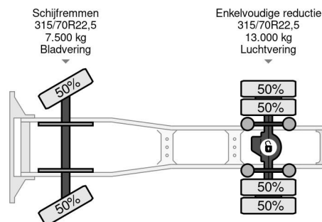
DAF XF 105.460 SPACECAB (4 IDENTICAL UNITS AVA... 4x2 Referentienummer: SN 58391679
