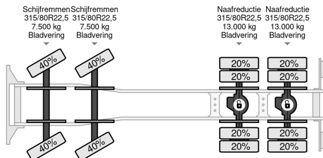
MAN 41.464 F2000 8X4 FULL STEEL KIPPER (EURO 2 / ZF... Referentienummer: SN 55149234 Z
