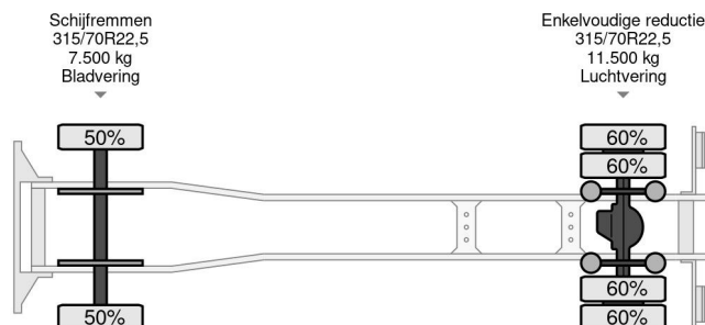
MAN TGM 18.250 BL WITH PLYWOOD CLOSED BOX ... 4x2 Referentienummer: SN 58577777
