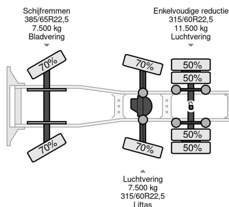
DAF 85.430 6x2 TRACTOR UNIT (EURO 4) (ZF16 MANUAL ...
