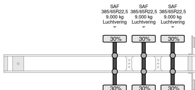
Feldebinder KIP48 3 3-AXLE 48M3 KIPPING SILO TRAILER (...)
